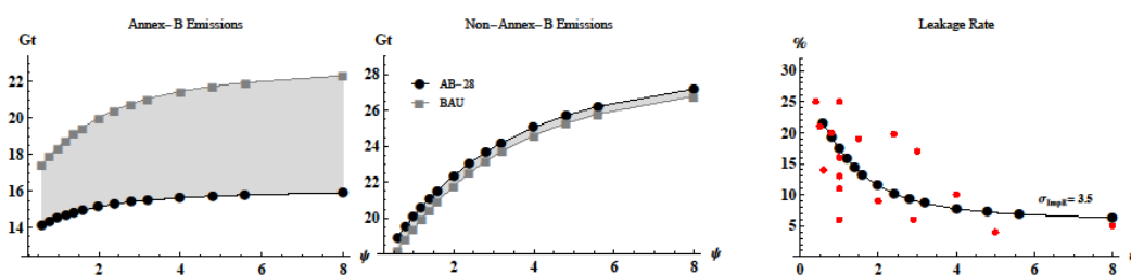
Figure 10: Sensitivity of leakage to \psi_{ES} for a $29/ton CO 2 tax in Annex B, no BTA's
